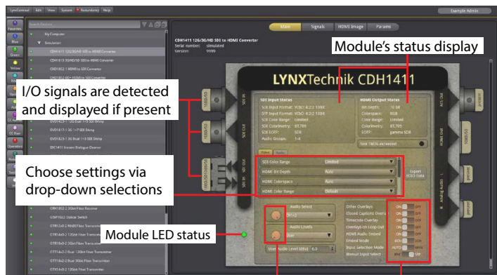
Controls marked in red indicate physical switches on the module. Status is indicated initially. Changes will prompt a warning.
