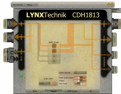
Controls marked in red indicate physical switches on the module. Status is indicated but cannot be changed via the software, unless enabled under settings.
