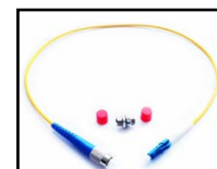
Model# LC/FC SIM LC/PC to FC/PC Adapter
