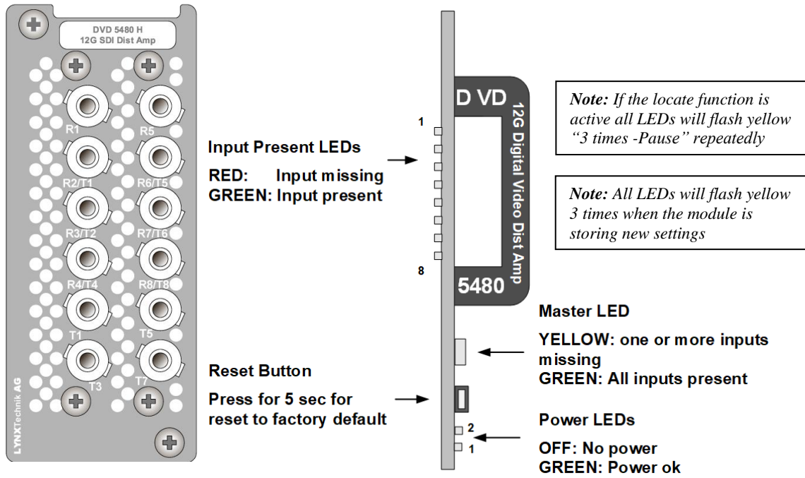
Termination Panel
