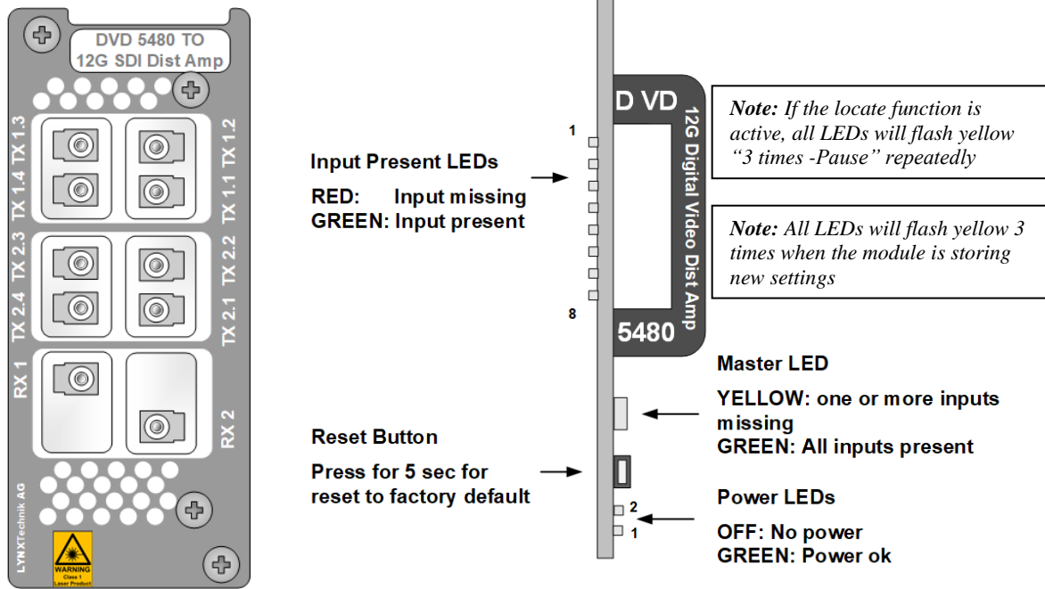
Termination Panel
